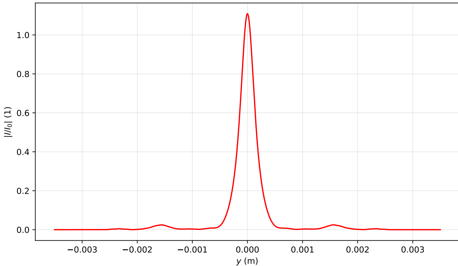
Intensity profile I(x = 0, y, z = 0.955)/I_0 , P_{in}=5.0P_{cr} , artificial time
